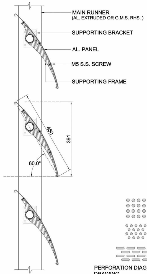
LENGTHWAYS SECTION
