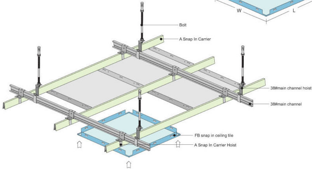
Structure and installation of FB snap in ceiling
